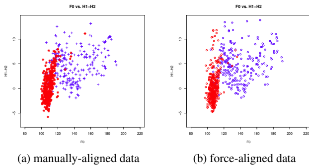
Figure 7: Scatter plot of F0 and H1-H2 for medial (blue) and final (red) ‘ta’ in manually aligned data (a) and force-aligned data (b).
